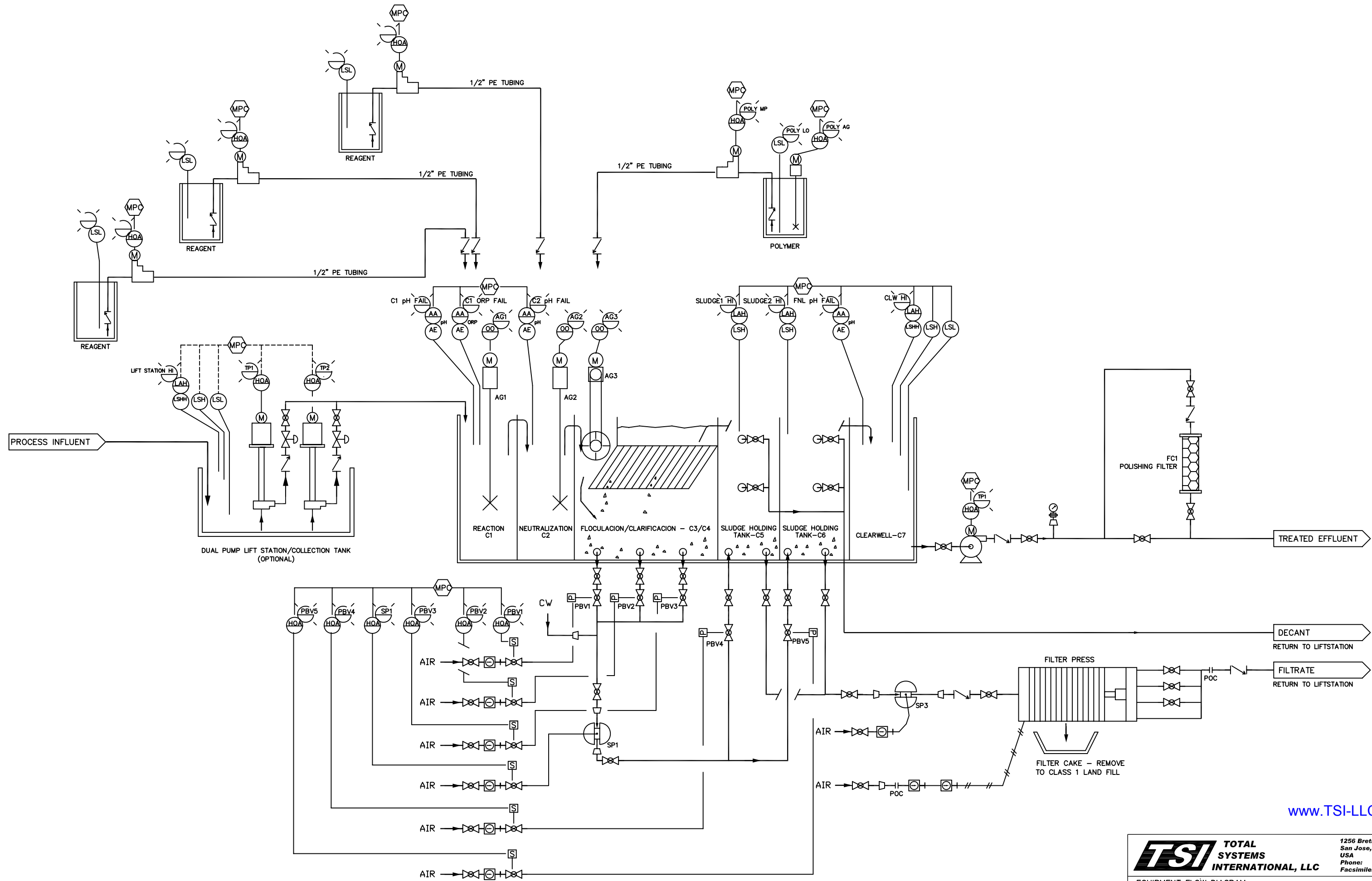
HMR - TWO CHAMBER PRECIPITATION SYSTEM
