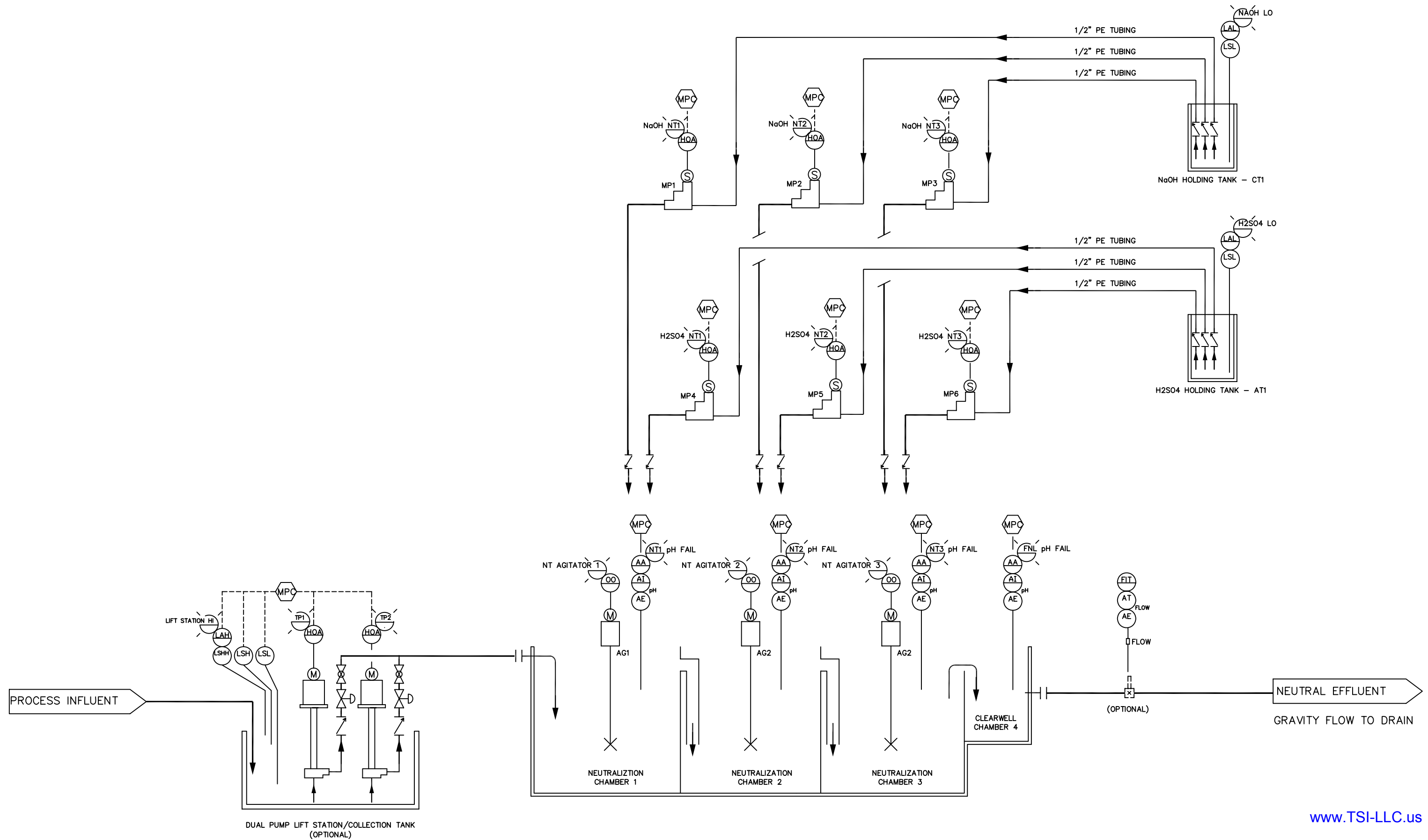
THREE STAGE NEUTRALIZATION SYSTEM
